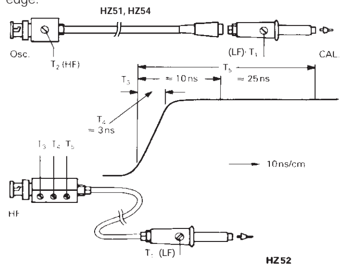
T_3 : alters the middle frequencies T_4 : alters the leading edge T_5 : alters the lower frequencies
